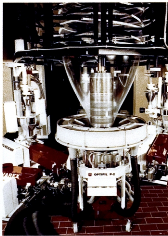
The industry's only automatic die: the OPTIFIL® P-2
